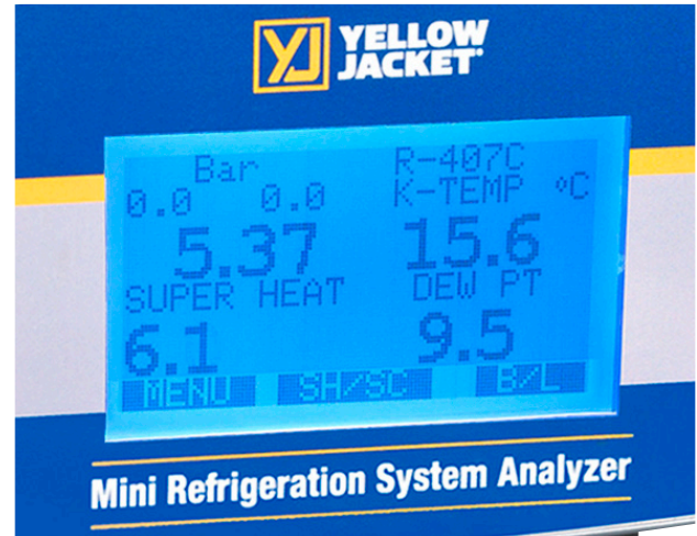
bar - Superheat
