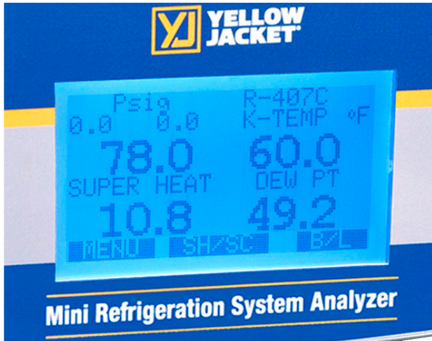
psi - Superheat
