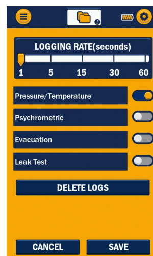
Figure 35: Logs Menu
