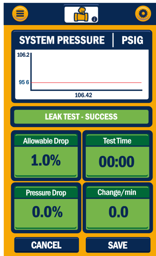
Figure 25: Pressure Decay Test - PASS
