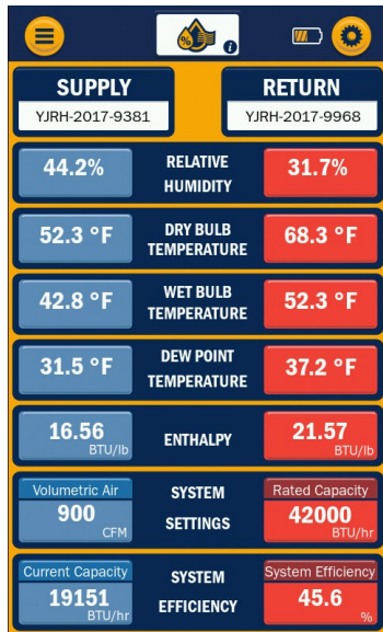
Figure 27: Psychrometric Menu
